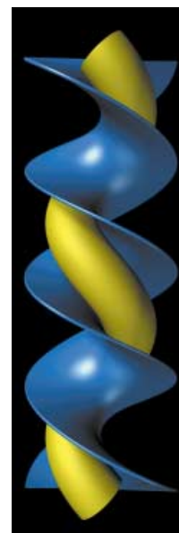
Figure 4. Schematic representation of a possible templating mechanism in which a coiled CdS helix is produced from a twisted helical template through growth along one face of the template. The resulting yellow mineral (shown at an early stage of growth so as not to obscure ribbon) would have a pitch twice that of the ribbon template (blue).
